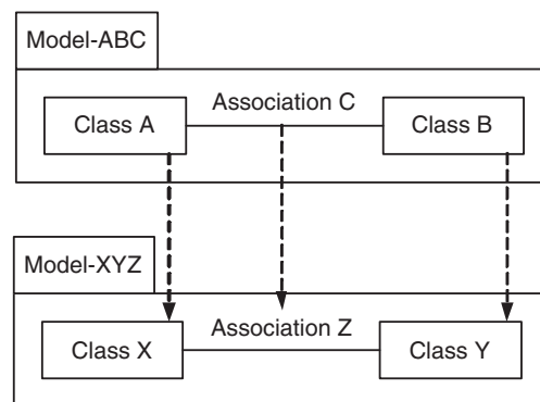
Figure 1. A common transformation kind.
