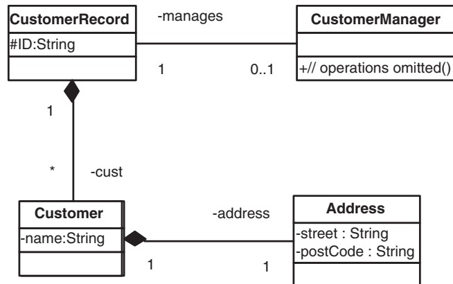
Figure 4. UML Class notation of example instance of the ECA Entity Model.
