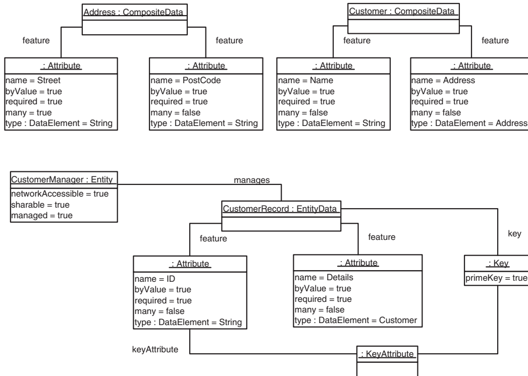
Figure 5. UML Object notation of example instance of the ECA Entity Model.
