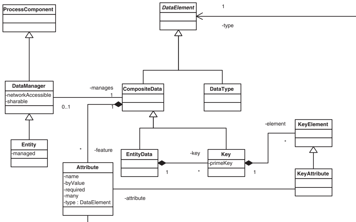
Figure 3. Part of the ECA Entity Model.
