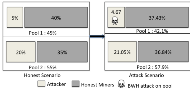
Fig. 2: Simple illustration of the BWH attack: if an attacker with 25% of the mining power of the network attacks Pool 1 with 5% of the network mining power, he gains 25.72% of the reward instead of the expected 25%.
