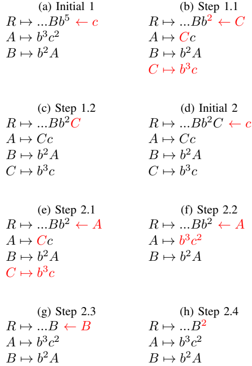
Fig. 3: PYTHIA-RECORD adding symbols in the grammar.
