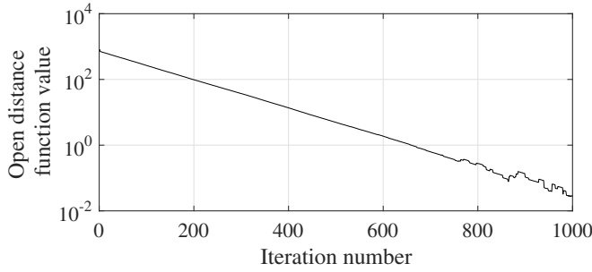
Fig. 3. Scenario A: Evolution of open distance function d(x(t), x_e(t)) .
