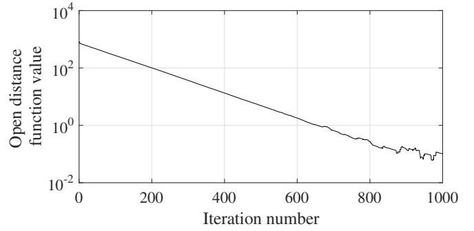
Fig. 7. Scenario B: Evolution of open distance function d(x(t), \bar{u}(t)) (estimation error).
