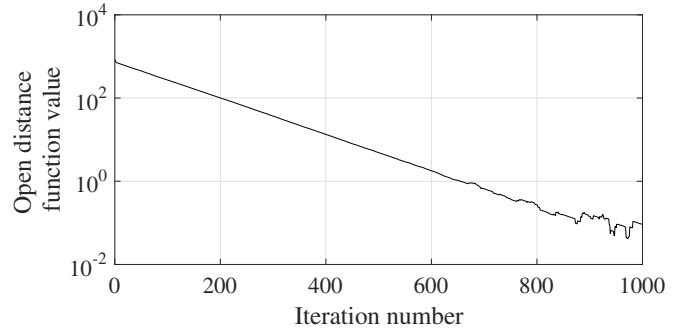
Fig. 6. Scenario B: Evolution of open distance function d(x(t), x_e(t)) .
