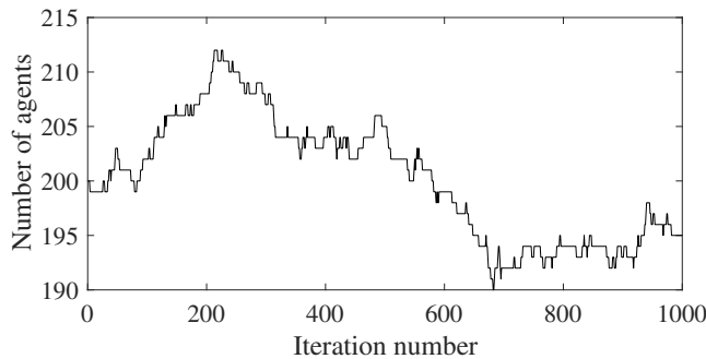
Fig. 5. Scenario B: Time-varying number of agents |V(t)|
