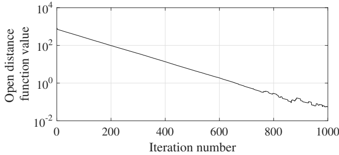
Fig. 4. Scenario A: Evolution of open distance function d(x(t), \bar{u}(t)) (estimation error).
