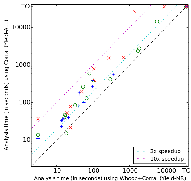
Fig. 9. Scatter plot showing the runtime speedups that CORRAL achieves using WHOOP with the Yield-MR instrumentation. The symbols +, o, and x represent a context-switch bound of 2, 5, and 9, respectively.
