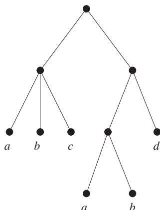
FIG. 2. A MUL-tree T with leaf label multiset \Lambda(T) = \{a, a, b, b, c, d\} = L and cluster collection \mathcal{C}(T) = \{\{a\}, \{a\}, \{b\}, \{b\}, \{c\}, \{d\}, \{a, b\}, \{a, b, c\}, \{a, b, d\}, L\} .
