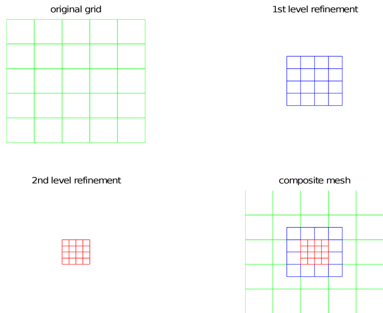
Figure 1. An example of overlapping block structured Cartesian mesh refinement. Two levels of refinement are applied to the local region.
