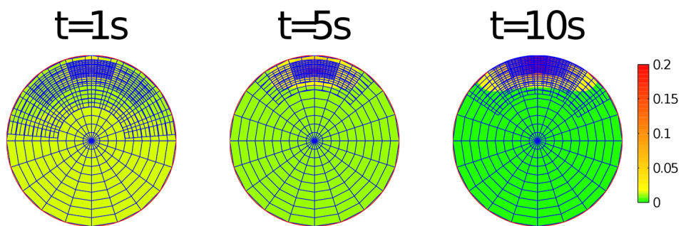
Figure 2. Contour plots for concentration of AB in the system (30) calculated using cIIF2 with AMR. The parameters for the simulation are D = 1\mu m^2 s^{-1} , k_{on} = 0.1(\mu Ms)^{-1} , k_{off} = 0.3s^{-1} , j_{on} = 1(\mu Ms)^{-1} , j_{off} = 0.005s^{-1} , j_{con} = 0.1(\mu Ms)^{-1} .
