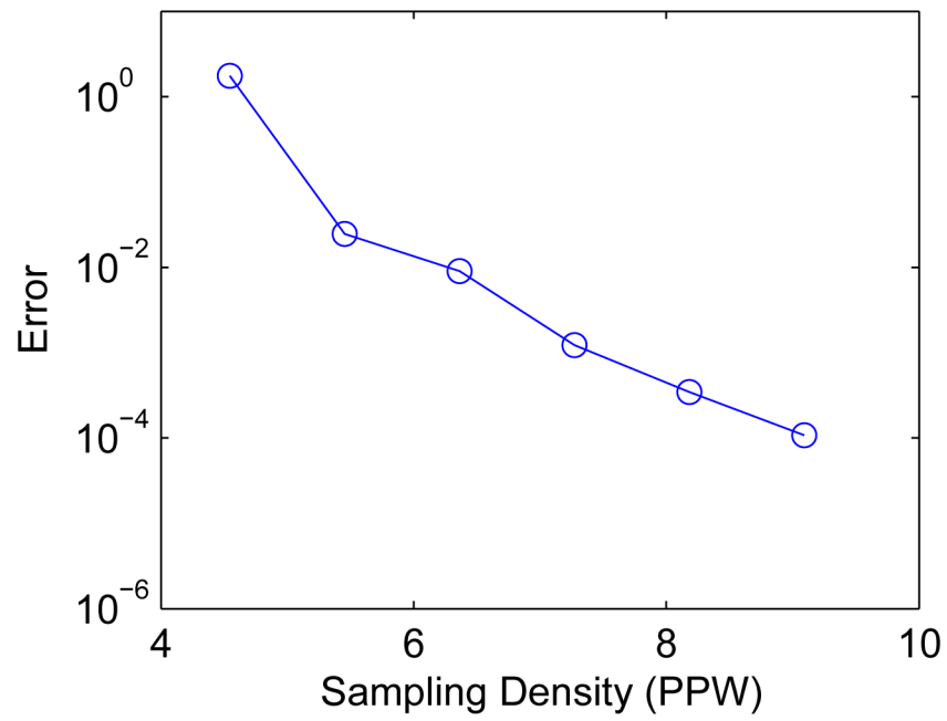
Fig. 9. The error of the wave function between numerical results and analytical solutions for a sphere quantum dot with plane wave incidence.
