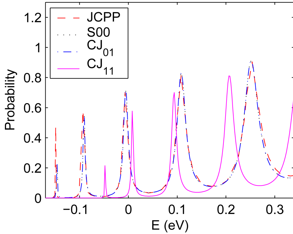
Fig. 13. The transmission coefficient comparison for a CNFET with different input energies and different incident waves.
