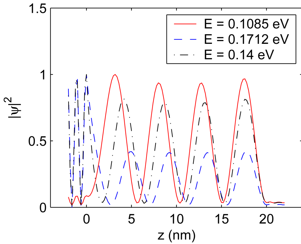
Fig. 14. The electron concentration along z direction of the coaxial CNFET with input energies E = 0.1085 eV, 0.1712 eV and 0.14 eV.
