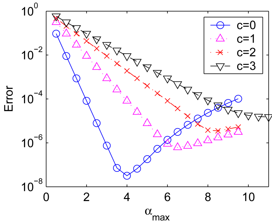
Fig. 5. The error convergence with the change of \alpha_{max} for c = 0 to c = 3 in the PML region.
