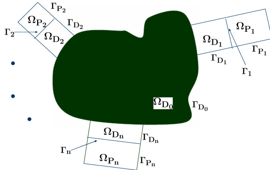
Fig. 1. The problem geometry for a semiconductor device with K contact regions truncated by the PML medium.
