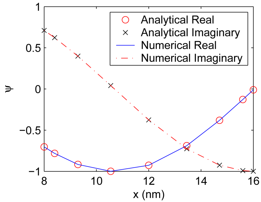
Fig. 4. Comparison of SEM results and analytical solutions for the wave components versus x at the center y and center z line in the device region.
