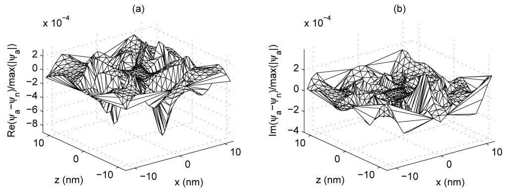
Fig. 8. The differences of the real (a) and imaginary (b) parts of the wave function at central y surface between numerical results and analytical solutions.
