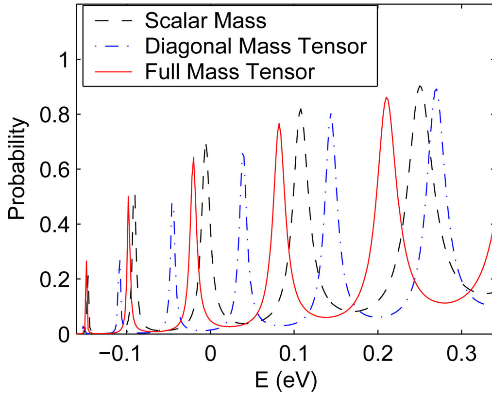
Fig. 15. Comparison of the transmission coefficient for three CNFETs with a scalar mass, diagonal mass tensor and full mass tensor versus the input electron energy.
