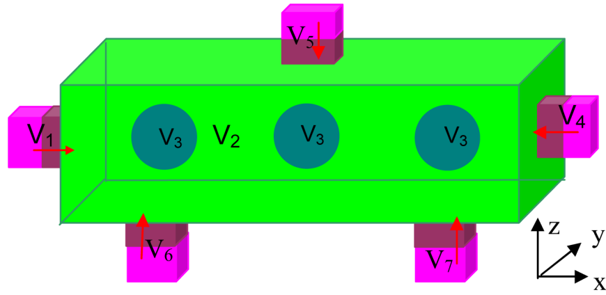
Fig. 10. The geometry for a device with three inner quantum dots, five incident terminals and five exit terminals.
