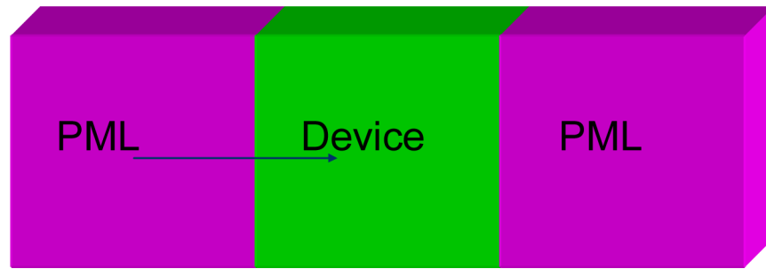
Fig. 3. The geometry for three-element PML Model.
