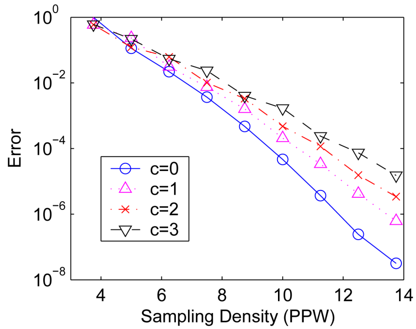
Fig. 6. The error convergence with the increase of the sampling density.
