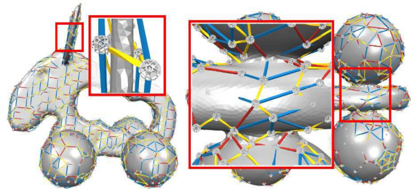
Figure 8. At the chosen resolution the antlers are thinner than y_0 and it is a difficult task to separate the “wheels” from the body of the ELK .
