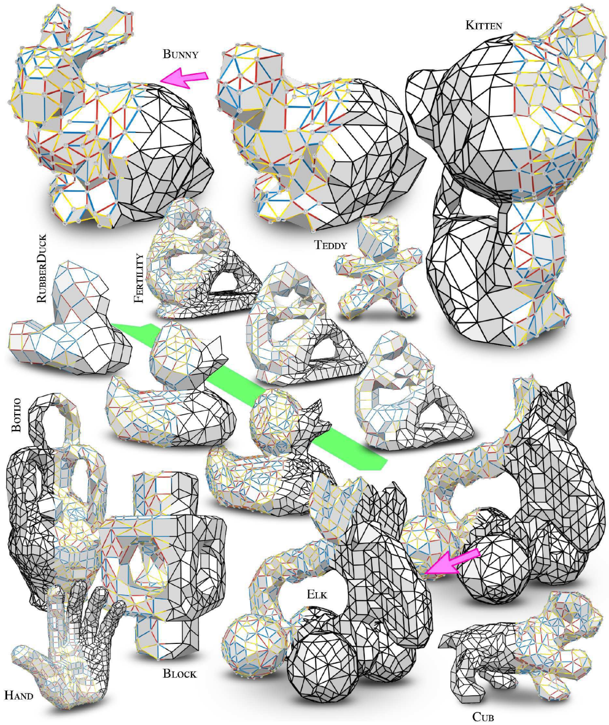
Figure 10. Resulting Zometool meshes. Along the green strip excerpts from a refinement and a decimation hierarchy are shown. At a coarse resolution the BUNNY and ELK both had details missing using the standard weights (pink arrow). By using the 3-step strategy to preserve thin features (discussed in Section 6) these details were successfully captured.
