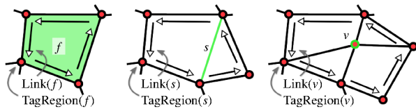
Figure 4. The TagRegion (red nodes) and oriented edges of the Link (arrows) of different mesh entities (green).
