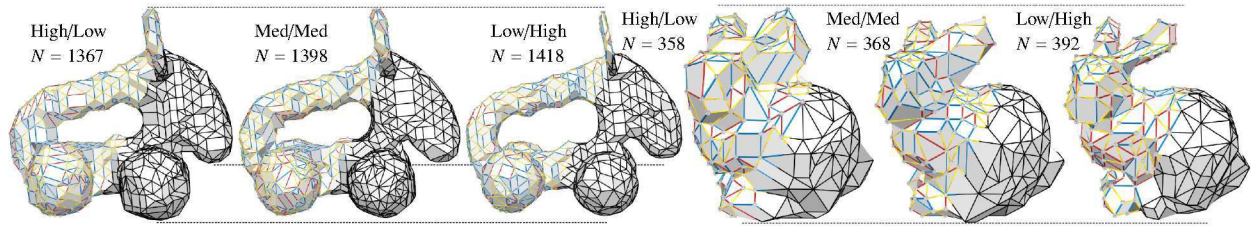
Figure 9. A 3-step scale of decreasing orientation weights and increasingly tightened forbidden zone weights (High/Low to Low/High) demonstrating how thin surface parts (ELK antlers and BUNNY ears respectively) can be preserved while still properly reaching concavities (e.g., between ELK wheels). The dotted lines show how high orientation tends to “bloat” the surface. Using the resulting N of the previous step as the new N_{\text{target}} also has a relaxing effect on the mesh complexity.
