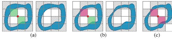
Figure 3. (a) depicts a non-manifold vertex (in 2D) and two adjacent simple cells in green, either can be removed to resolve the configuration while preserving the genus. In (b) the red cell is no longer simple, as its removal would change the genus, however, the green cell can still be removed. Finally, (c) depicts a configuration that cannot be resolved by this approach.
