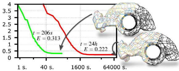
Figure 6. The top ROCKERARM is obtained after about 3min with a final energy of 0.313, while the bottom result is obtained after 24h with a final energy of 0.222.
