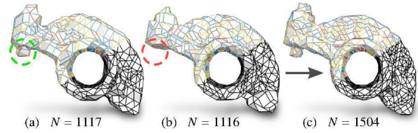
Figure 7. (a) and (b) demonstrate how using SA the same weights can sometimes lead to slightly different results. Once a good solution exists, further passes can be used to refine the result (b)→(c).
