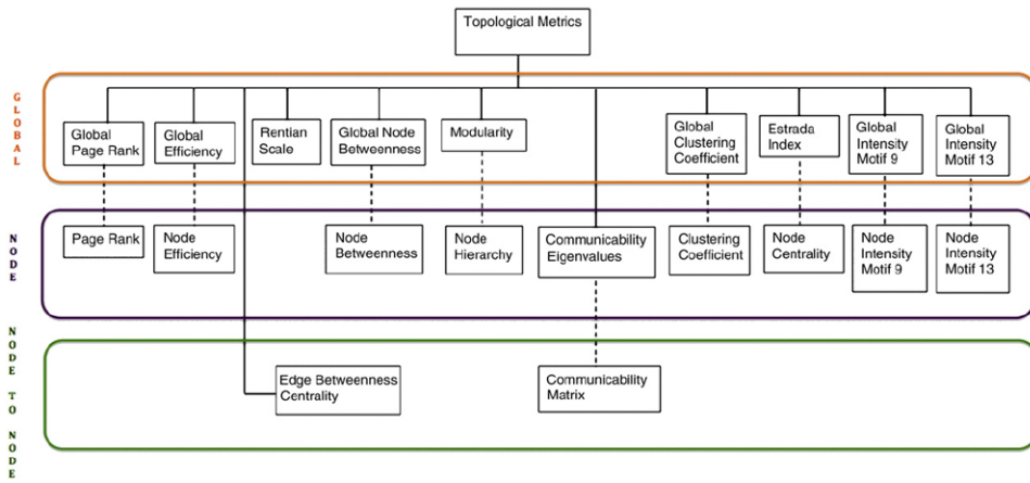
Fig. 1. Hierarchy of multiple families of hypothesis testing.
