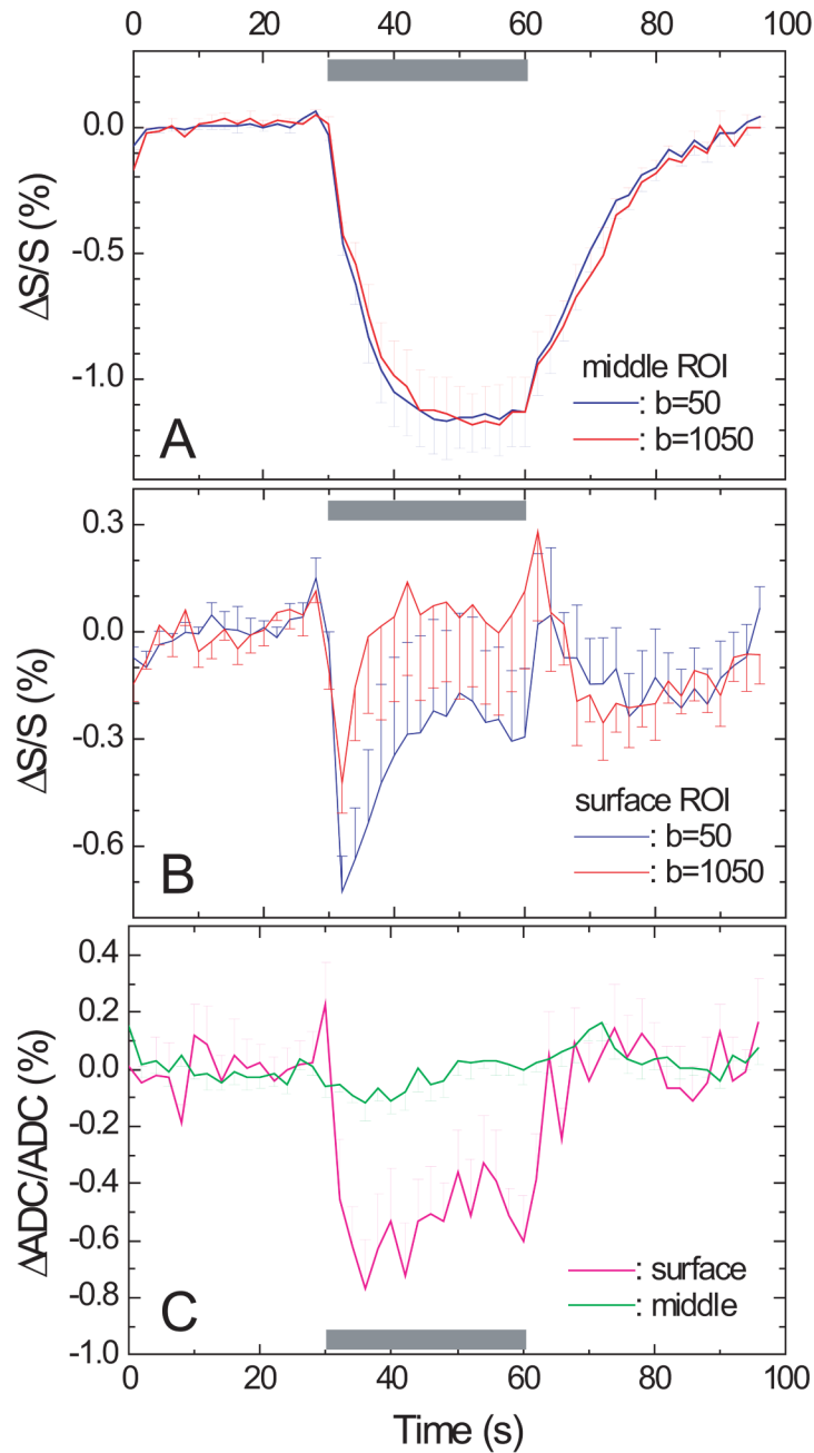
Fig. 5. Average time courses ( n = 7 animals) of fMRI data with MION. (A and B): DW fMRI data at the middle cortical ROI (A) and surface ROI (B). (C) average ADC time courses ( n = 7 ) at both ROIs. Decreased ADC changes were detected at the cortical surface, which may have been induced by a partial volume change of CSF. Gray bars: stimulation period; error bars: standard errors of means.
