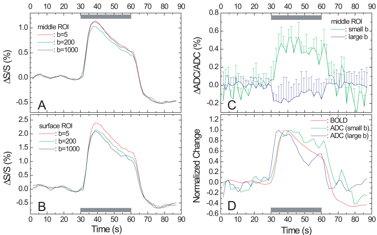
Fig. 3. Average time courses ( n = 6 ) of fMRI data without MION. Three DW fMRI time courses were obtained from the middle cortical ROI (A) and surface ROI (B). The average ADC time course from the middle cortical ROI (C) showed an increase in ADC for the small b -value pair, but a decrease for the large b -value pair. To compare dynamic properties, BOLD (from b = 5 \text{ s/mm}^2 ) and ADC time courses at the middle cortical ROI (D) were normalized by its corresponding peak and smoothed by a three-point temporal average. Gray bars: stimulation period; error bars: standard errors of means.
