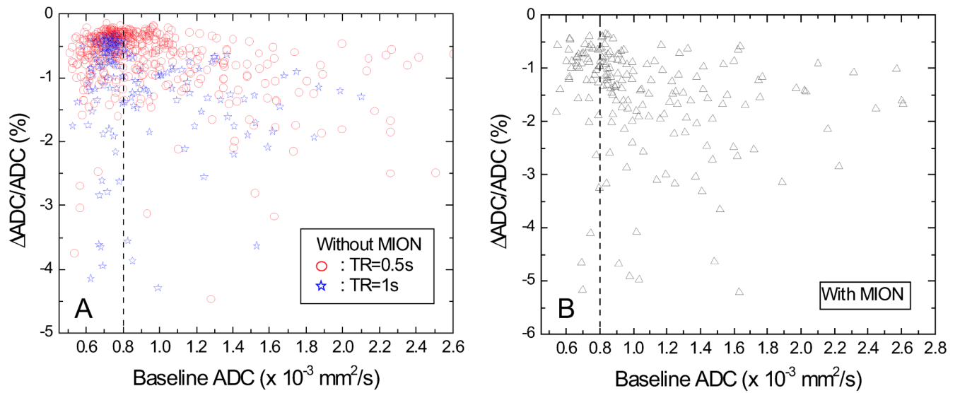
Fig. 6. Sites of functional ADC-decreasing pixels. (A and B): Scatter plot of ADC change versus baseline ADC value for ADC-decreasing pixels without (A) and with (B) MION injection. Without MION, 51.4% and 60% of negative pixels were inside the parenchyma (with baseline \text{ADC} \leq 0.8 \times 10^{-3} \text{ mm}^2/\text{s} , indicated by a vertical dashed line) for TR = 0.5 s (n = 6) and 1 s (n = 3) data, respectively. With MION (n = 7), 27% of pixels were in the parenchyma.
