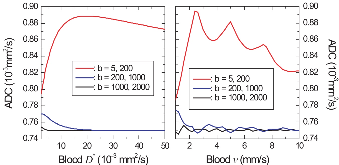
Fig. 7. Simulated ADC values as a function of blood pseudo-diffusion coefficient (A) and blood velocity (B). ADC values were calculated based on Eq. [2], assuming CBV = 3\% and tissue D = 0.75 \times 10^{-3}/\text{mm}^2 . Three ADC values were calculated from b -value pairs of 5 and 200 \text{s}/\text{mm}^2 (red), 200 and 1000 \text{s}/\text{mm}^2 (blue), and 1000 and 2000 \text{s}/\text{mm}^2 (black).
