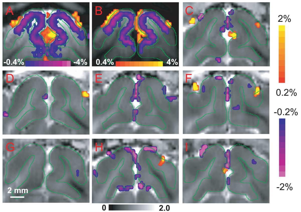
Fig. 4. Functional maps of all seven animals after the removal of intravascular signals with MION. Percentage change maps for DW-fMRI with b = 50 (A) and b = 1050 s/mm 2 (B) and the corresponding ADC fMRI change map (C) were obtained from one representative animal. Gray matter areas were outlined in green. The color bar for DW-fMRI maps is shown in (A) and (B). Horizontal grayscale bars: baseline ADC values in units of 10^{-3} mm 2 /s; color bar on right: percentage ADC changes. (D-I) ADC percentage change maps from the other six animals, overlaid on corresponding baseline ADC images. The activated pixels appeared mostly on the cortical surface.
