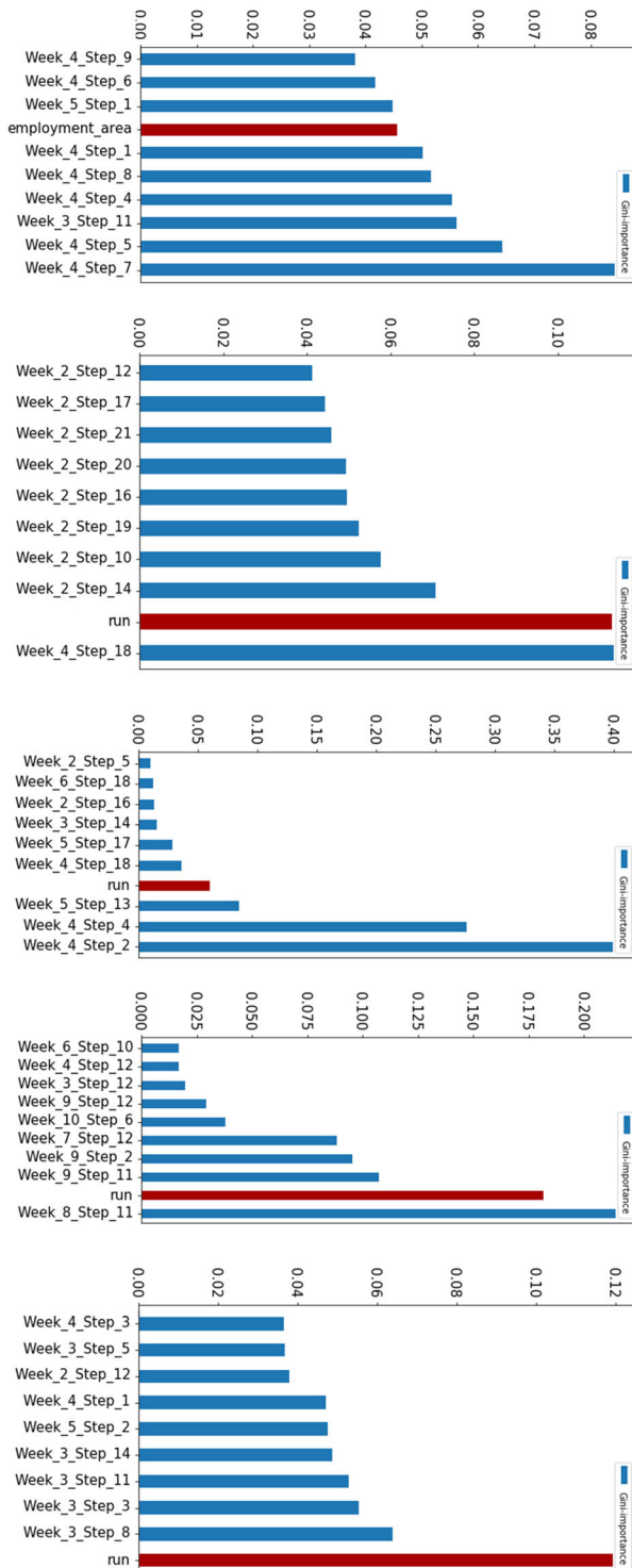
Fig. 2 The Most Representative Features for Predicting Course Purchasing Behaviour
