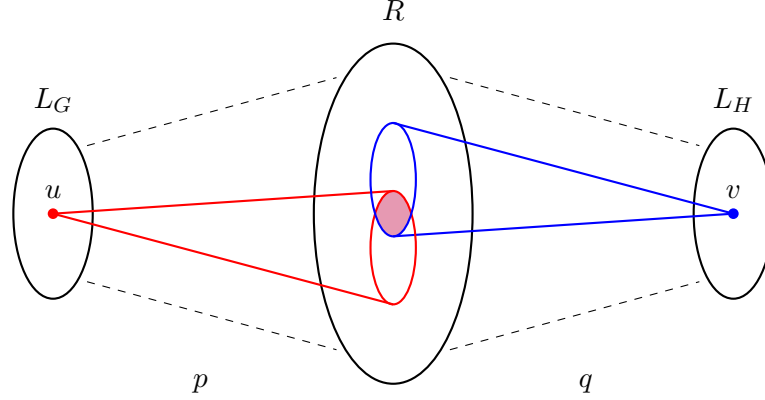
Figure 1: Random bipartite graphs \tilde{G} and \tilde{H} .
