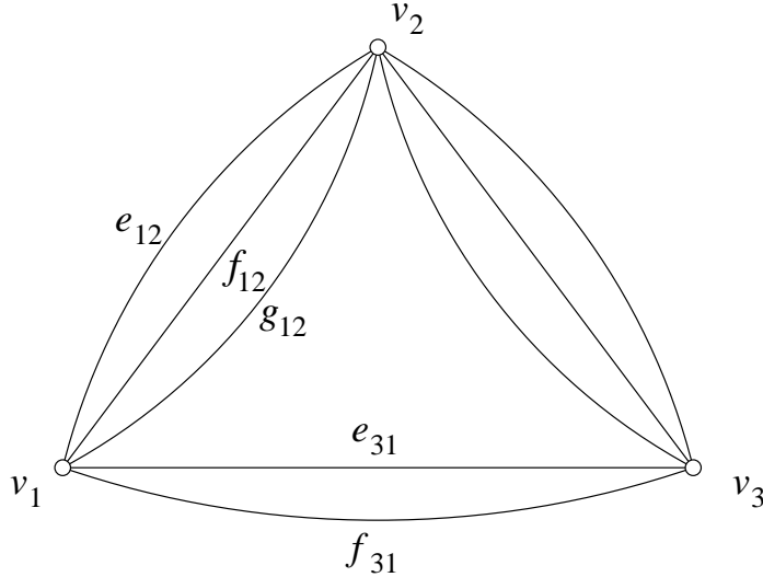
Figure 1: C_3(3, 3, 2) for Example 1 and Proposition 6.10.
