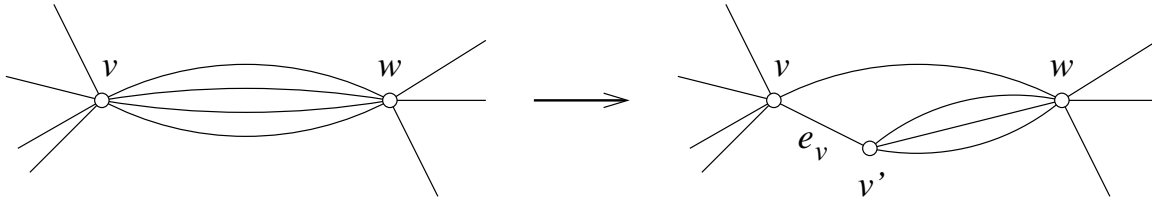
Figure 2: Extruding an edge from v .
