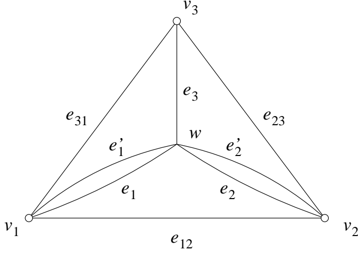
Figure 3: The edge labels of K_4'' .
