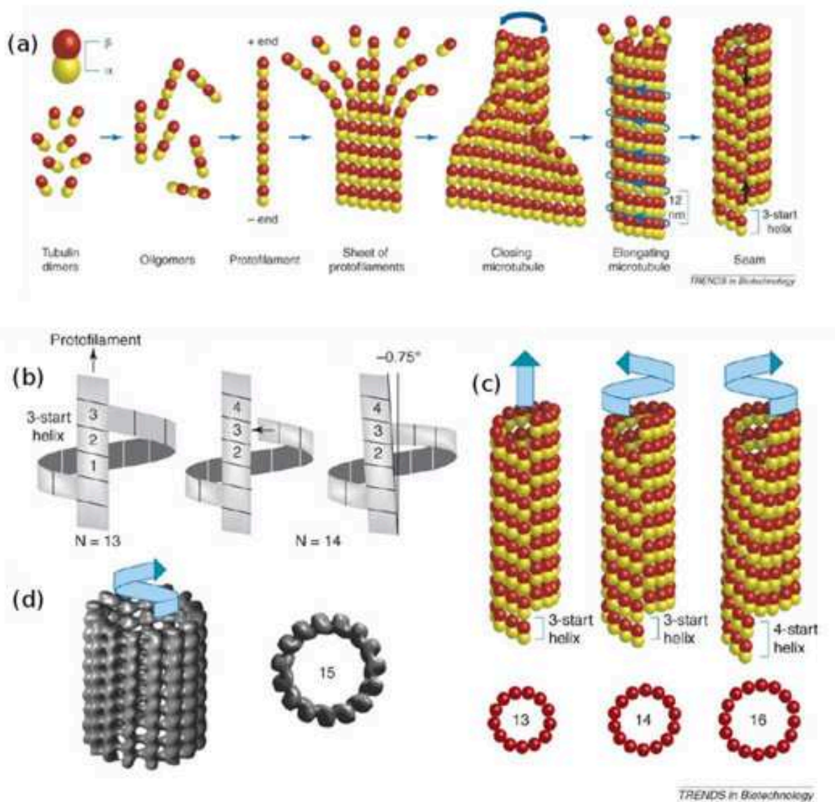
Figure 1.3: (a) Schematic description on self-assembly of MTs. \alpha - and \beta - tubulin dimers assemble into straight protofilament in alternative manner. The PFs start to interact laterally forming a sheet with characteristic intrinsic inward curvature, and the sheet closes into a tube forming a microtubules. (b) Depending on the number of PFs, MTs has different helical surface lattices, (c) 14- and 16-PFs MTs are left- and right-handed lattice, respectively. (d) Isosurface rendering of the electron density of a 15-PFs MTs are shown to have right-handed helical lattice [73].
