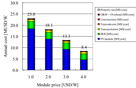
Fig. 10 Annual cost for a 100 MW tracking VLS-PV system
