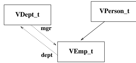
(a) Schematic of view entities and relationships
