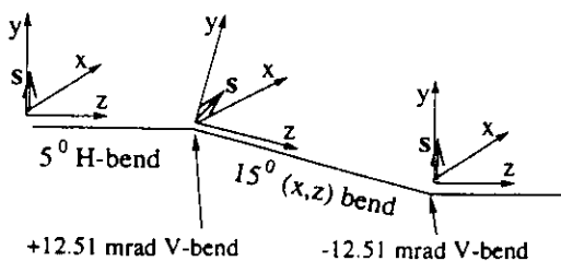
Fig. 1. Diagram of the "12.5 mrad vertical bend".
