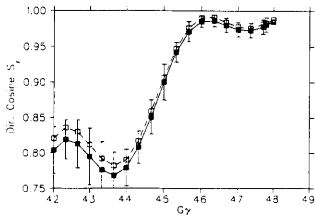
Fig. 3. S_y component of the stable spin direction at RHIC injection point. AGS partial snake off.
