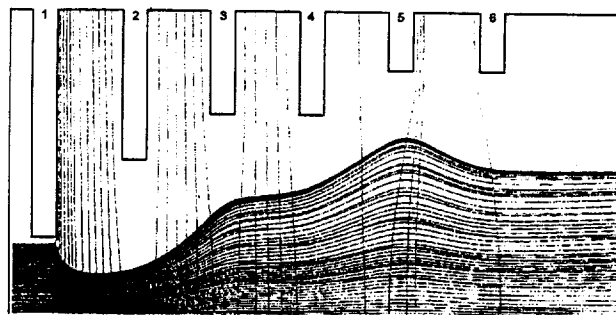
Figure 2 : LEBT layout and beam envelope
