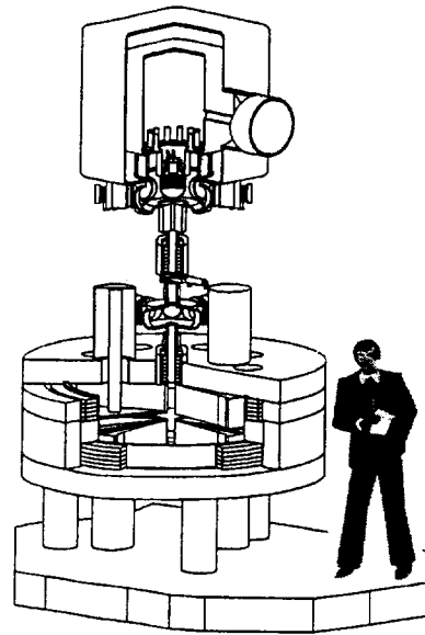
Figure 1 :View of the injector
