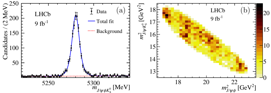
Figure 1: (a) Invariant-mass distribution of selected B^0 candidates and corresponding fit result. (b) Distribution of m_{J/\psi K_S^0}^2 versus m_{J/\psi\phi}^2 for candidates in the \pm 15 MeV region around the nominal B^0 mass.
