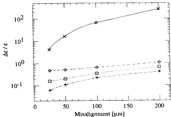
Fig. 2 Emittance dilution versus BPM resolution and misalignment magnitude for 4 cases: (solid) 1-to-1 correction only, (dashes) method (d) with \sigma_{res} = 2.0 \mu\text{m} , (dots) method (d) with \sigma_{res} = 1.0 \mu\text{m} , and (dash-dot) method (d) with \sigma_{res} = 0.5 \mu\text{m}
