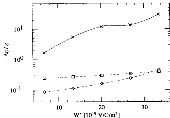
Fig. 1 Emittance dilution versus wakefield strength for 3 cases: (solid) no correction, (dashes) correction varying charge and bunch length, and (dots) correction varying only charge; in the SLAC NLC design, W' = 7 \times 10^{19} \text{ V/C/m}^3 .
