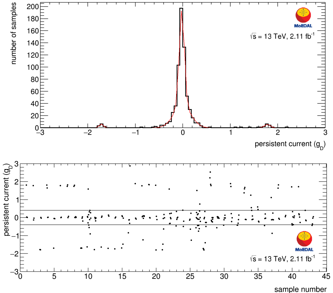
FIG. 1. Top: persistent current (in units of g_D after application of a calibration constant) after first passage through the magnetometer for all samples. The red curve shows a fit of the measured distribution using a sum of four Gaussian functions. Bottom: results of repeated measurements of candidate samples with absolute measured values in excess of 0.4g_D .
