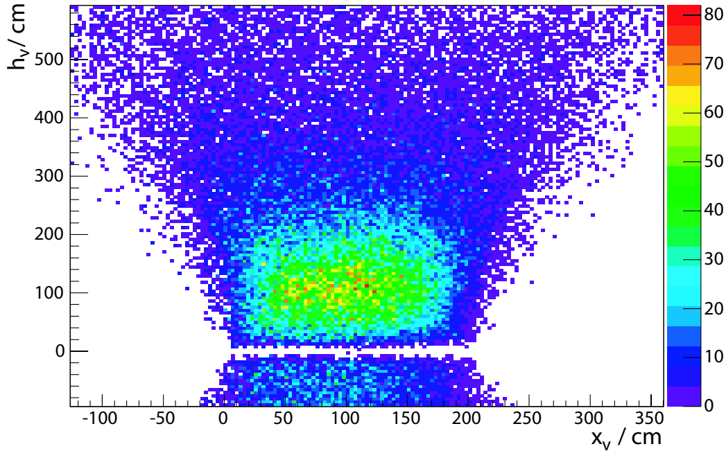
Figure 9.3: Reconstructed vertices of double tracks. The superlayer lies in the horizontal gap at a height h_v of 0 cm. The vertices are accumulated about one metre above the superlayer.
