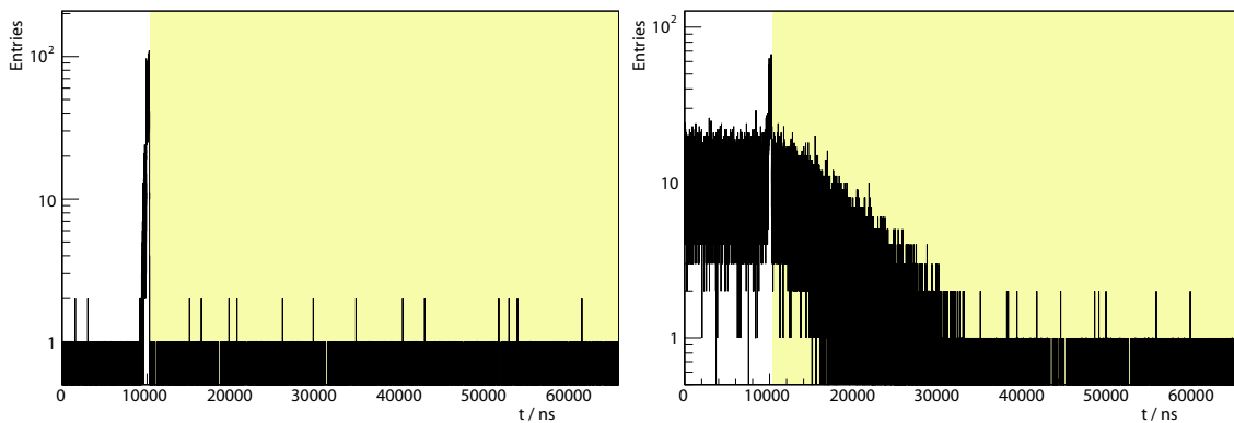
Figure 8.3: Shaded is the region of the complete TDC spectrum where all hits are regarded as noise. The usual drift time region appears as a peak around 10,000 ns. The left spectrum shows a cell with a normal noise rate, the right one has a noise rate of some 10 kHz which lets the spectrum drop as the TDC ring buffers can not store more than 16 hits.
