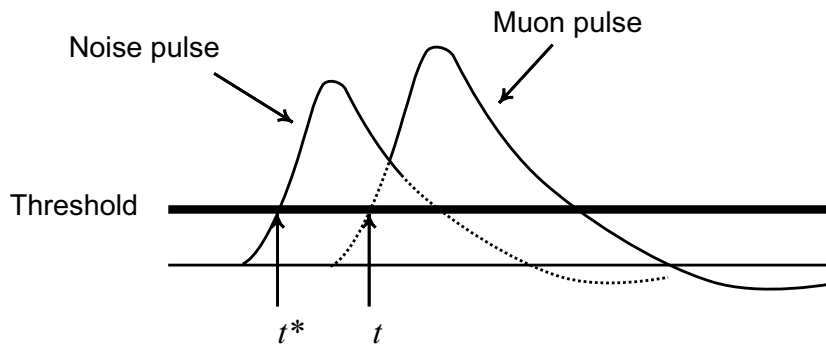
Figure 8.1: A noise hit masks a muon pulse. As the noise signal does not fall below the threshold amplitude before the arising muon pulse the latter is not registered. Its time t seems to be shifted to t^* < t [28].
