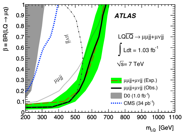
Fig. 5 95 % CL exclusion region resulting from the combination of the \mu\mu jj and \mu\nu jj channels shown in the \beta versus leptoquark mass plane. The shaded area at the left indicates the D0 exclusion limit [14] and the thick dotted line indicates the CMS exclusion region [13]. The dotted and dotted-dashed lines indicate the individual limits derived for the \mu\mu jj and \mu\nu jj channels, respectively. The combined observed limit is indicated by the solid black line. The combined expected limit is indicated by the dashed line, together with the solid band containing 68 % of possible outcomes from pseudo-experiments in which the yield is Poisson-fluctuated around the background-only expectation
