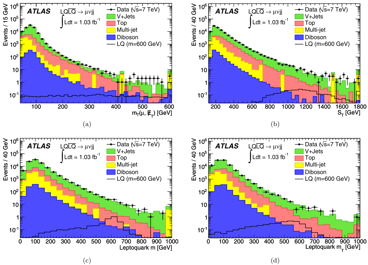
Fig. 2 Distributions of the input LLR variables for the \mu\nu jj channel for data and the SM backgrounds. (a) Transverse mass of the muon and the E_T^{\text{miss}} in the event, (b) S_T , (c) LQ mass, and (d) LQ transverse mass. The stacked distributions show the various background contributions,
