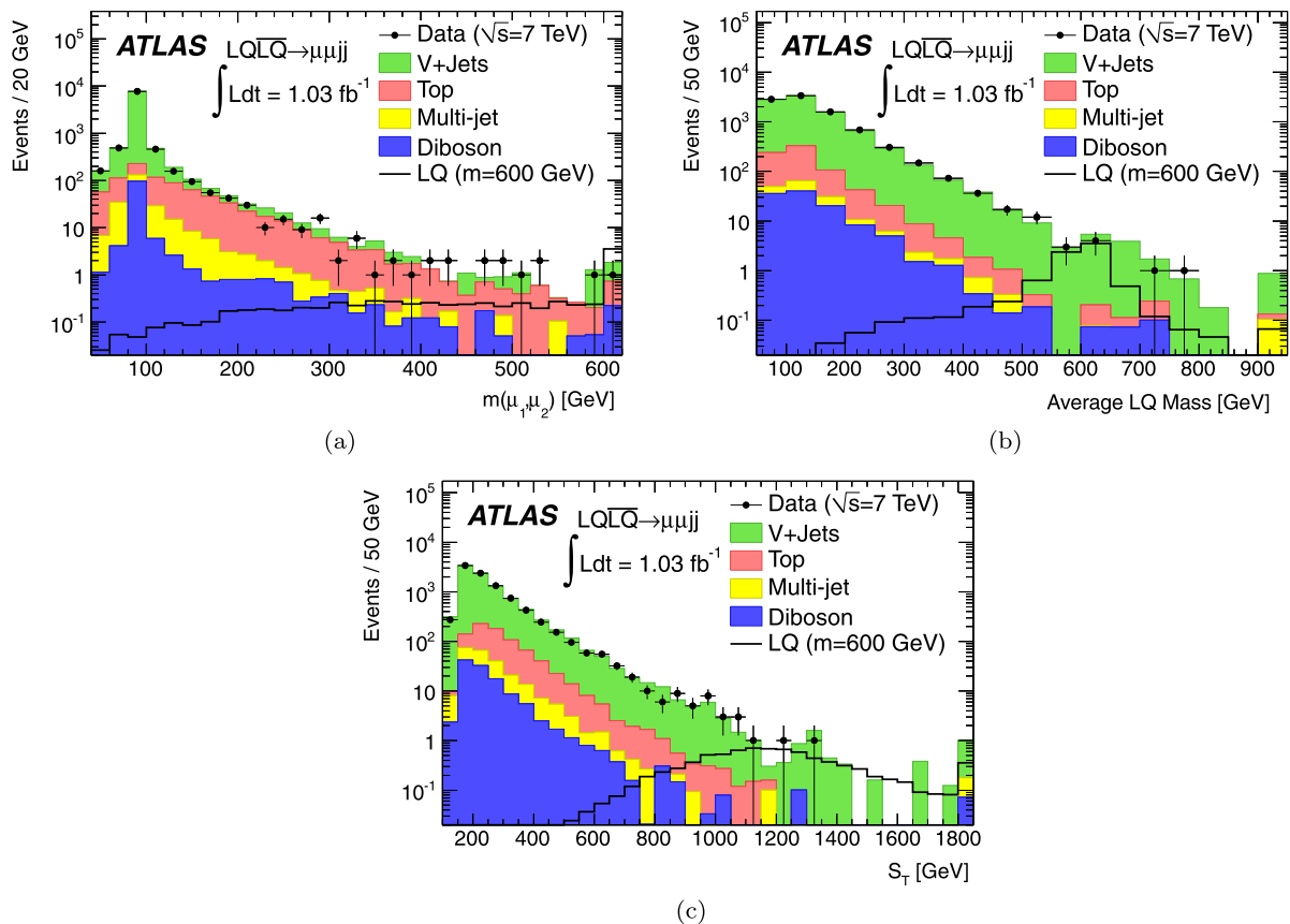
Fig. 1 Distributions of the input LLR variables for the \mu\mu jj channel for data and the SM backgrounds. (a) Invariant mass of the two muons in the event, (b) Average LQ mass resulting from the best muon-jet combinations in each event, and (c) S_T . The stacked distributions
