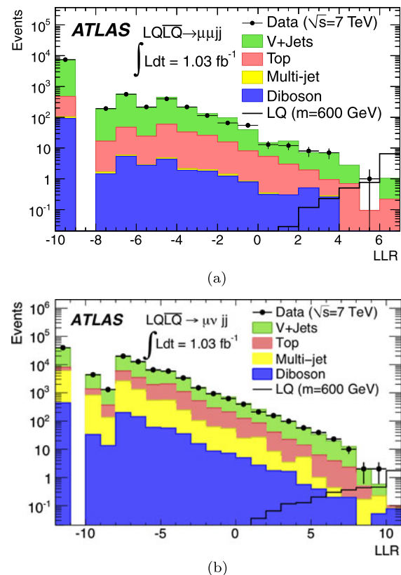
Fig. 3 (a) LLR distributions for the \mu\mu jj and (b) for the \mu\nu jj final states for a LQ mass of 600 GeV. The data are indicated with the points and the filled histograms show the SM background. The multi-jet background is estimated from data, while the other background contributions are obtained from simulated samples as described in the text. The LQ signal corresponding to a LQ mass of 600 GeV is indicated by a solid line, and is normalized assuming \beta = 1.0 (0.5) in the \mu\mu jj ( \mu\nu jj ) channel. The lowest bin corresponds to background events in regions of the phase space for which no signal events are expected
