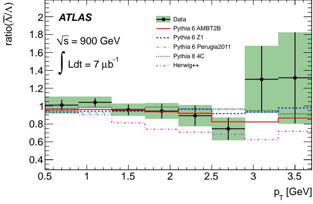
FIG. 23. The production ratio between \bar{\Lambda} and \Lambda baryons in 900 GeV data versus p_T . The error bars show the statistical uncertainties while the band shows statistical and systematic uncertainties added in quadrature.
