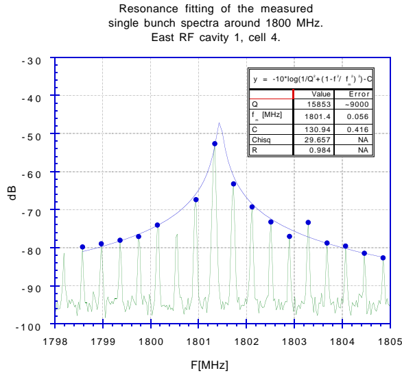
Figure 4: Resonance fitting of spectrum around TM0-ME-3 mode location. E1 cavity, cell 4.
