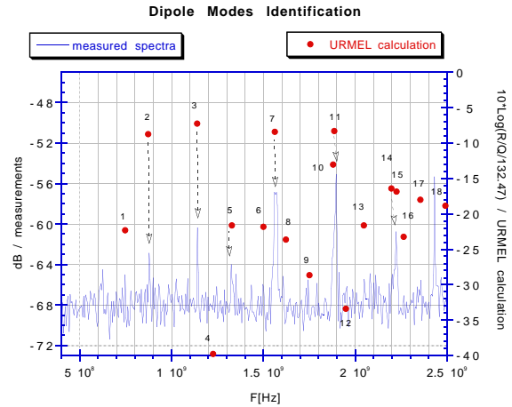
Figure 3: Dipole modes identification.
