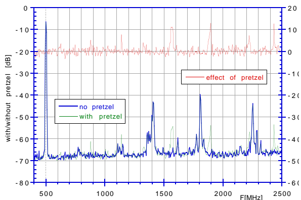
Figure 1: Spectra of signal from field probe of E1 cavity cell 4.
