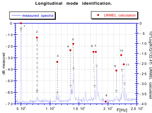
Figure 2: Longitudinal modes identification.
