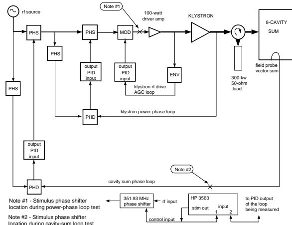
Figure 1: The rf system layout and closed-loop response measurement setup.
