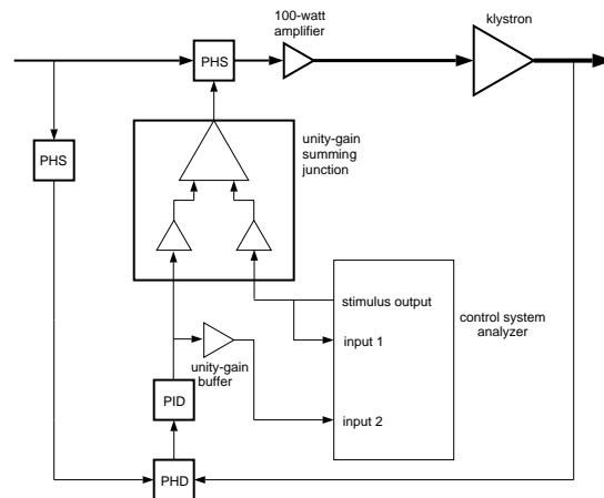
Figure 2: Setup for measuring open-loop characteristics.
