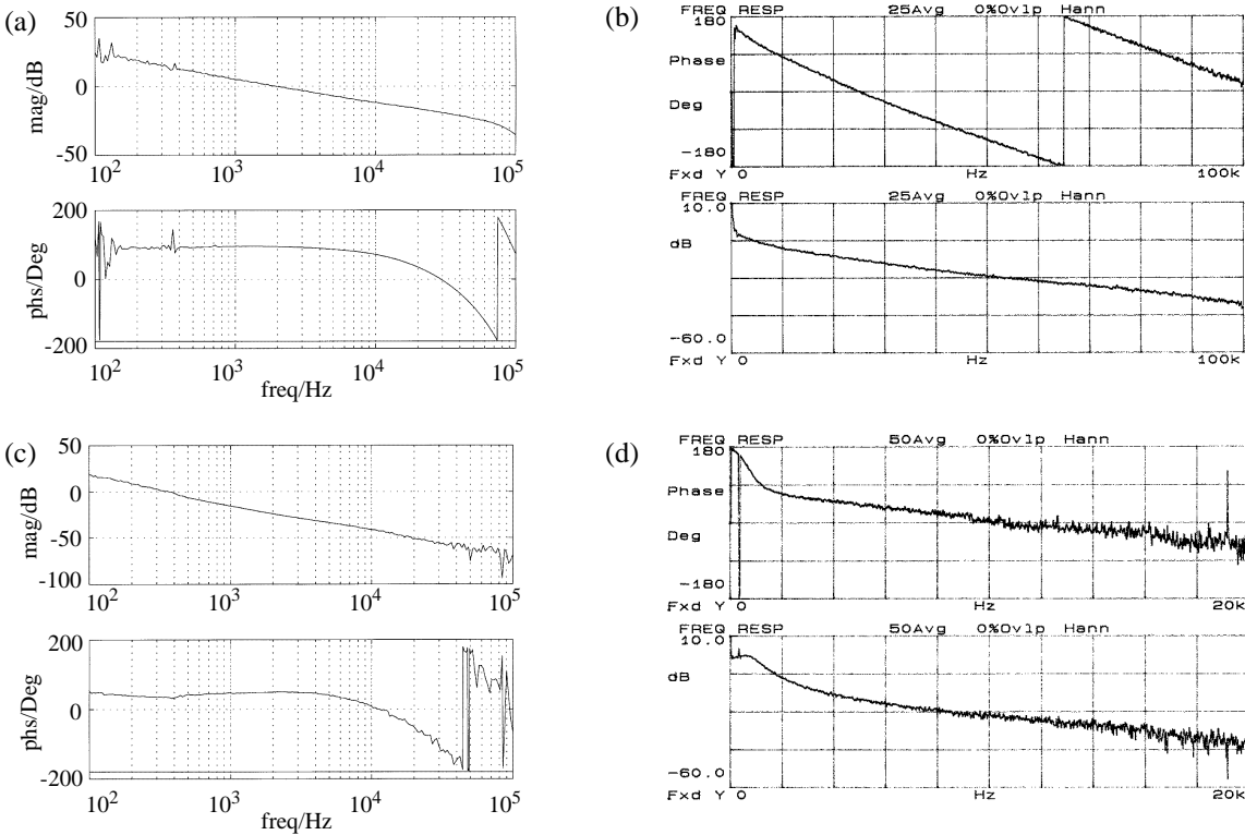
Figure 4: (a) Power-phase loop open-loop characteristics using SFT method; (b) power-phase loop open-loop characteristics using FFT method; (c) cavity-sum phase loop open-loop characteristics using SFT method; (d) cavity-sum phase loop open-loop characteristics using FFT method.
