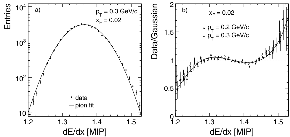
Fig. 6 (a) Conventional Gaussian fit of the MTPC dE/dx distribution, for tracks with pion selection using the VTPC dE/dx ; (b) ratio of data and fit function
