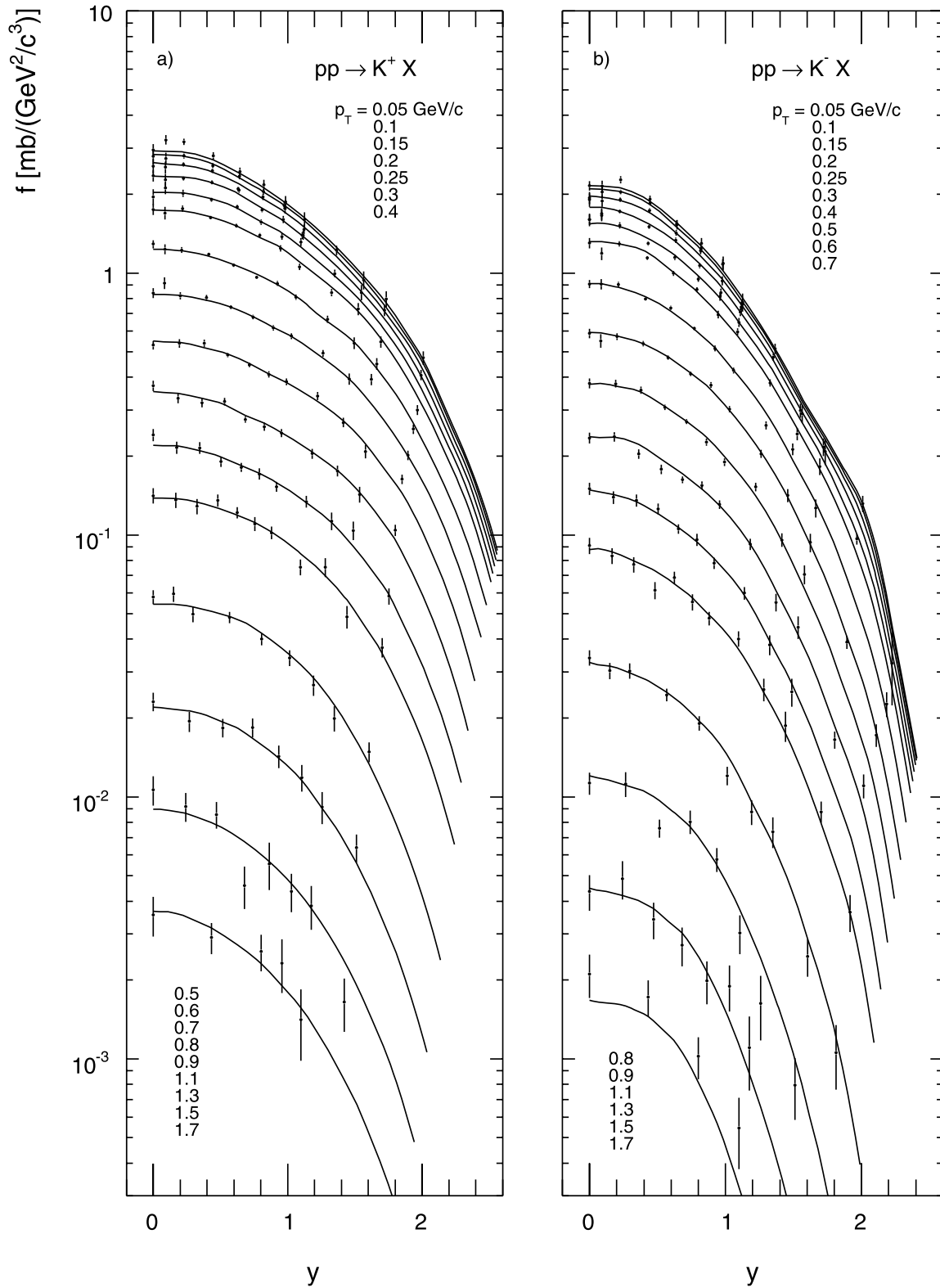
Fig. 23 Double differential invariant cross section f(x_F, p_T) [ \text{mb}/(\text{GeV}^2/c^3) ] as a function of y at fixed p_T for (a) K^+ and (b) K^- produced in p+p collisions at 158 GeV/c beam momentum. The lines show the result of the data interpolation, Sect. 6.2
