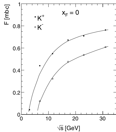
Fig. 70 F(x_F = 0) for K^+ and K^- as a function of \sqrt{s} for 6 different energies
