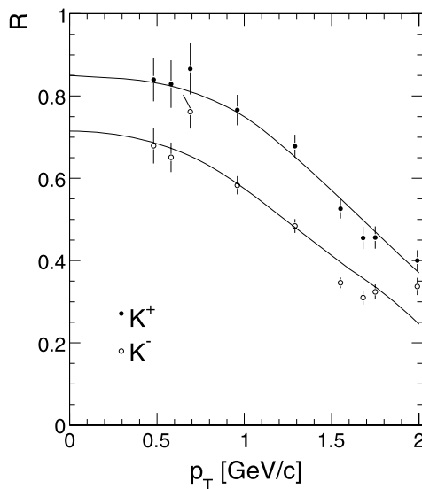
Fig. 69 Cross section ratio R of [11] to NA49 for K^+ and K^-
