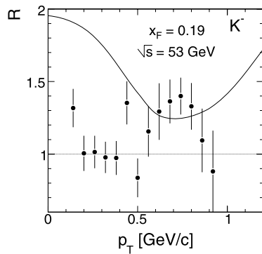
Fig. 83 Ratio R between [16] and NA49 for K^- at x_F = 0.19 as a function of p_T . The full line gives the behaviour at x_F = 0
