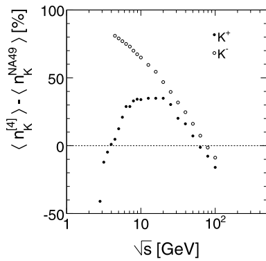
Fig. 133 Relative deviations between the present study of charged kaon yields and [4] in percent as a function of \sqrt{s}
