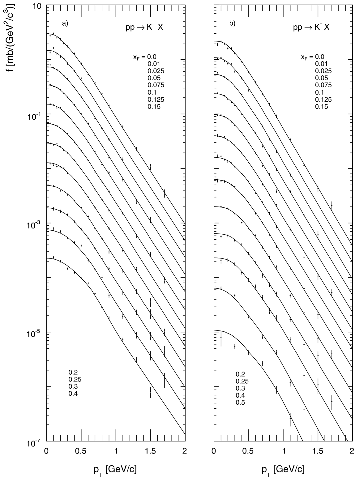
Fig. 21 Double differential invariant cross section f(x_F, p_T) [mb/(GeV 2 /c 3 )] as a function of p_T at fixed x_F for (a) K + and (b) K - produced in p + p collisions at 158 GeV/c beam momentum. The dis-
