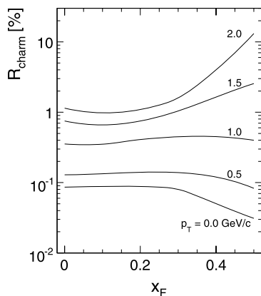
Fig. 128 R_{\text{charm}} as a function of x_F for fixed values of p_T , in %
