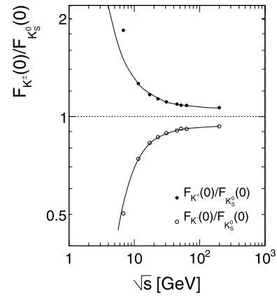
Fig. 135 Ratio between K^+ and interpolated K_S^0 data (full circles) and between K^- and interpolated K_S^0 data (open circles) as a function of \sqrt{s}
