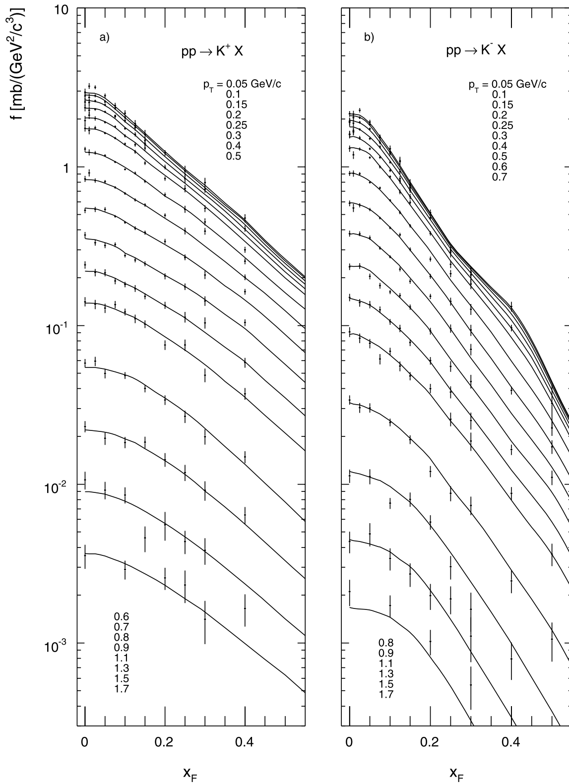
Fig. 22 Double differential invariant cross section f(x_F, p_T) [ \text{mb}/(\text{GeV}^2/c^3) ] as a function of x_F at fixed p_T for (a) K^+ and (b) K^- produced in p + p collisions at 158 GeV/c beam momentum. The lines show the result of the data interpolation, Sect. 6.2
