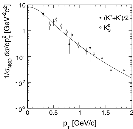
Fig. 106 UA5 data at \sqrt{s} = 540 GeV. The full line corresponds to the fit described in the text
