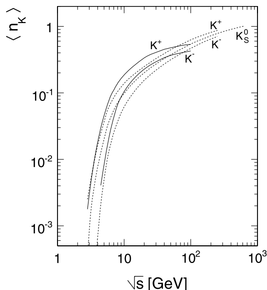
Fig. 132 \langle n_{K^+} \rangle and \langle n_{K^-} \rangle from [4] as a function of \sqrt{s} , full lines, compared to the interpolated K^+ , K^- and K_S^0 yields Fig. 130 (broken lines)
