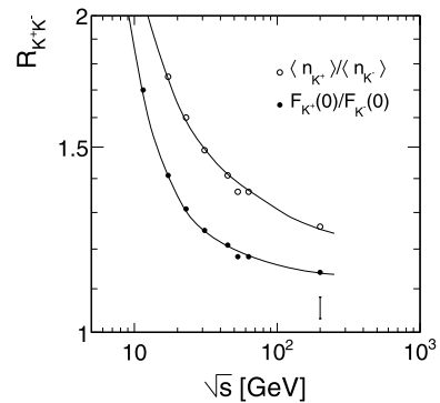
Fig. 136 R_{K^+K^-} ratios for total yields (open circles) and F(x_F = 0) (closed circles) as a function of \sqrt{s} . The error bar at \sqrt{s} = 200 GeV marks the range of F_{K^+}(0)/F_{K^-}(0) of published results by the RHIC experiments
