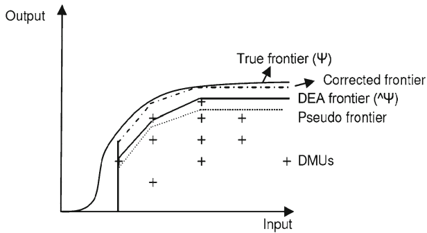
Fig. 3 Bootstrap idea (2)
